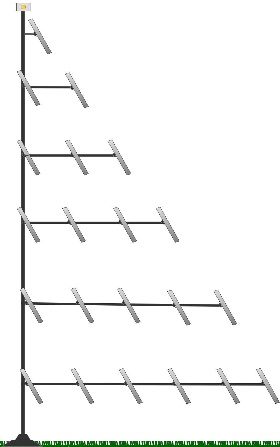
Vertical Solar Trees
